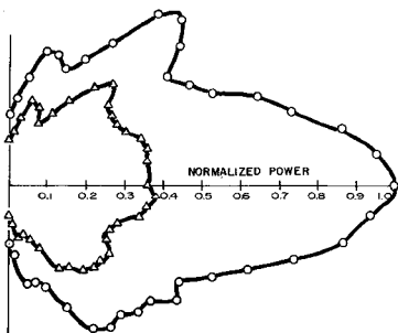
FIG. 6 EXPERIMENTAL RADIATION PATTERNS FOR ○—○ FEATHER ARRAY AND WAVEGUIDE (TUNED) □—□ FEATHER ARRAY AND WAVEGUIDE (UNTUNED) △—△ WAVEGUIDE WITH NO FEATHERS (TUNED)
